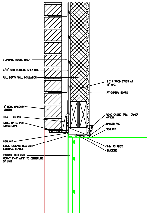
HEAD DETAIL
