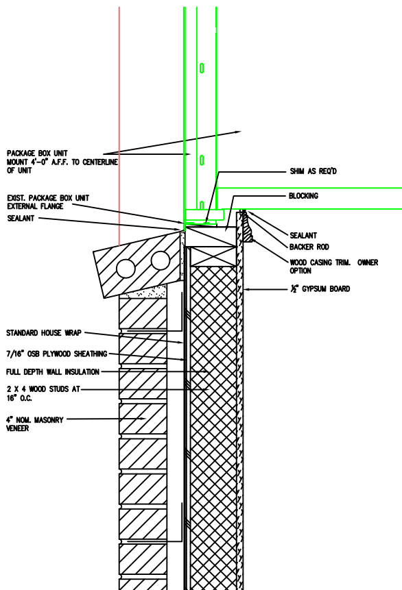
SILL DETAIL
